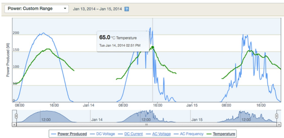
Figure 1: Enphase M215 Microinverter internal temperature data (14/1/2014)
